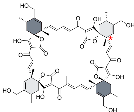
FIGURE 4 : Structure de la quartromicine
